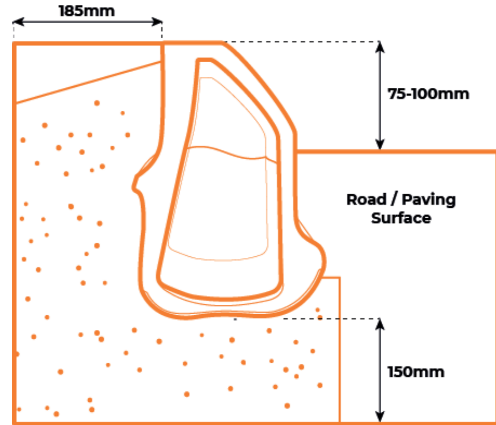
PolyKerb - Splay
